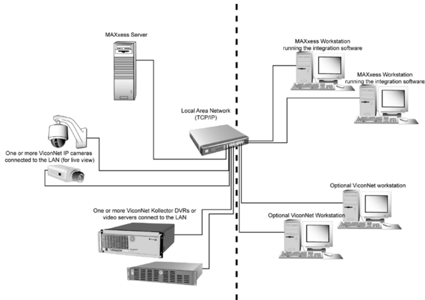
Typical MAXxess/ViconNet Network Setup
